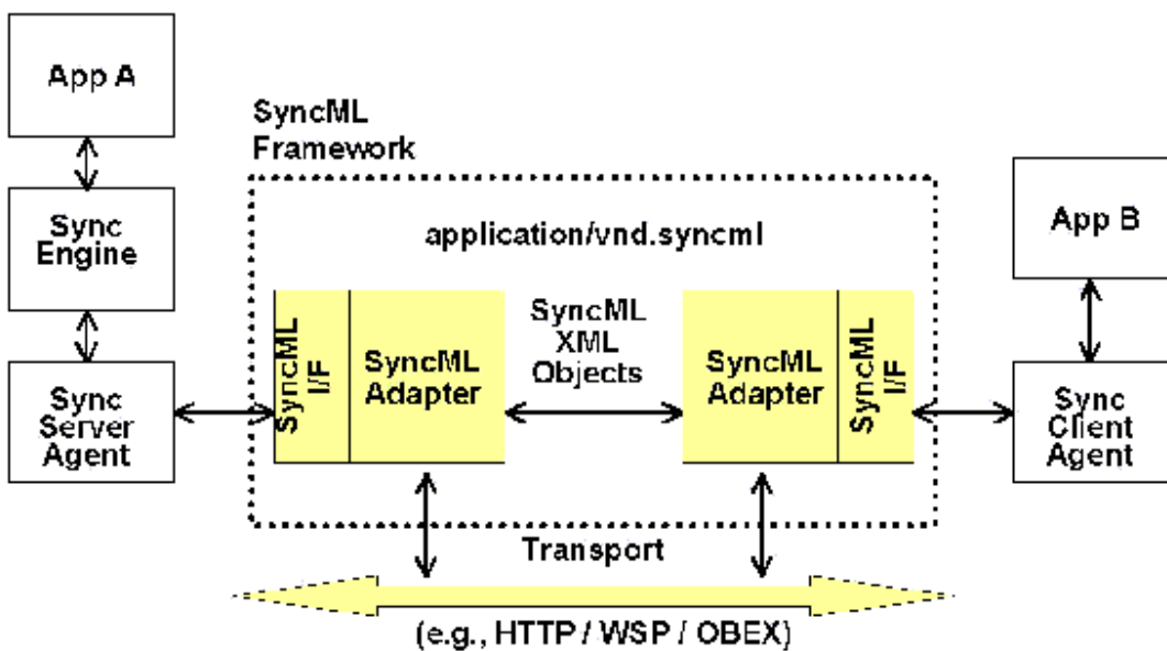
Figure 2 SyncML Framework
