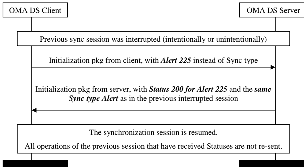
Figure 9: Resume mechanism
