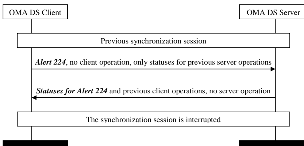
Figure 8: Suspend mechanism
