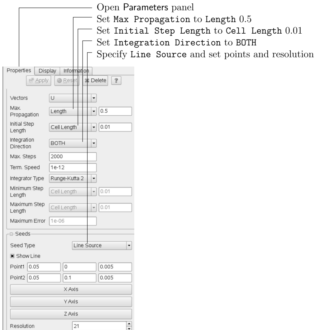
Figure 2.8: Properties panel for the Stream Tracer filter.
