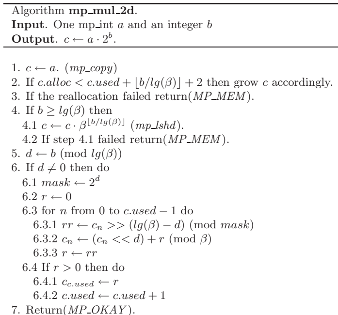
Figure 4.12: Algorithm mp_mul_2d
