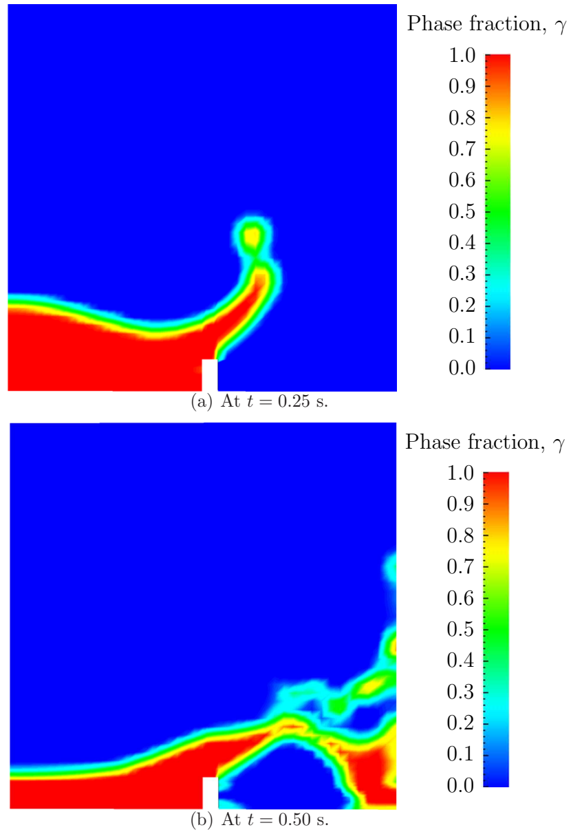
Figure 2.22: Snapshots of phase \gamma .
