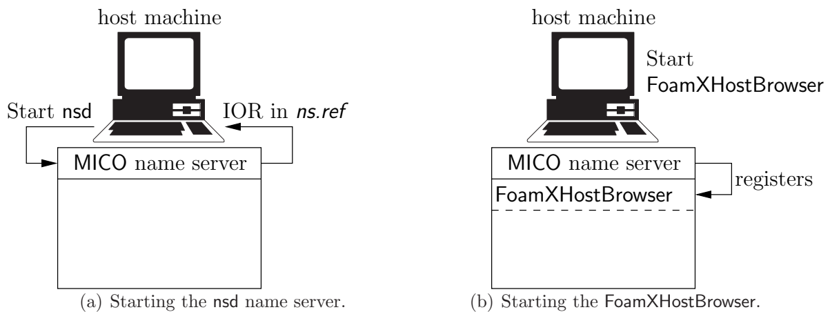
Figure A.2: Running runFoamXHB.
