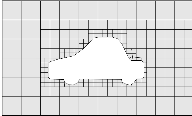
Figure 5.15: Surface snapping in snappyHexMesh meshing process
