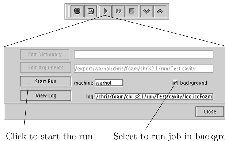
Figure A.20: Running a solver using the Start Calculation function
