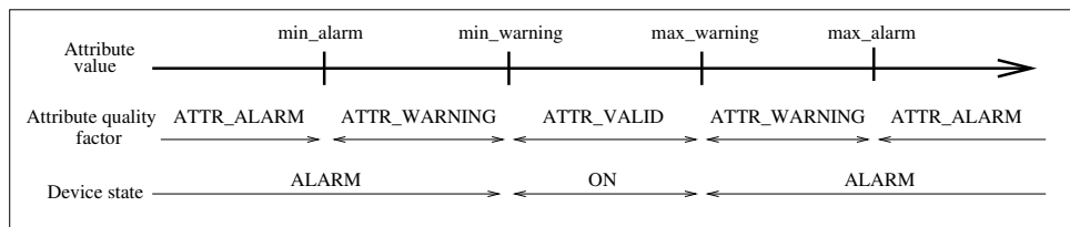
Figure 9.1: Level alarm
