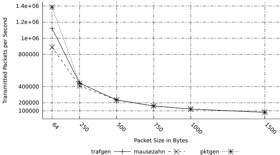
Comparison of Traffic Generators
